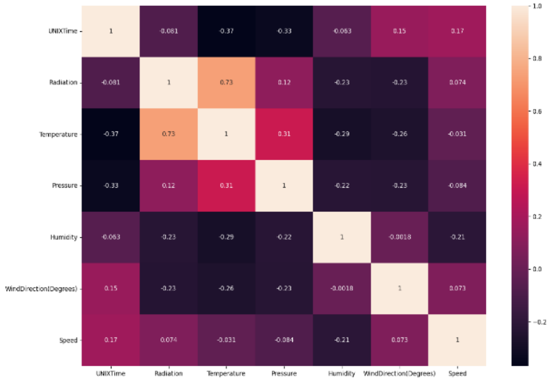
Figure 12: Correlation Matrix.
